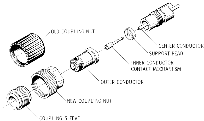
New and Old Coupling Nuts for APC-7 Connectors
